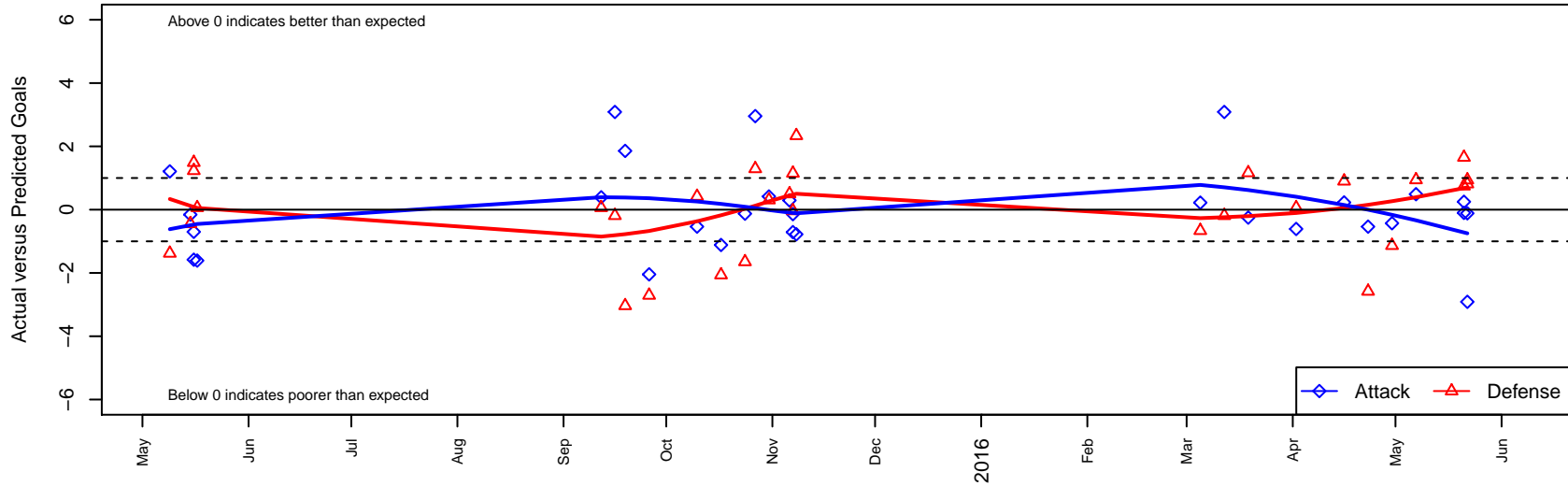
Idaho Rush Grey B03 Dots are actual minus expected GF (blue circles) and GA (red triangles). Blue line is smoothed change in attack strength. Red is smoothed change in defense strength.
